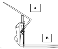
A – Lowback Forks will float and pivot up B – Highback Forks will float only
